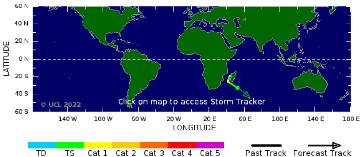
Figure 3: No tropical storm risk observed on 30 January 2023.
